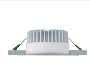
Installation detail
